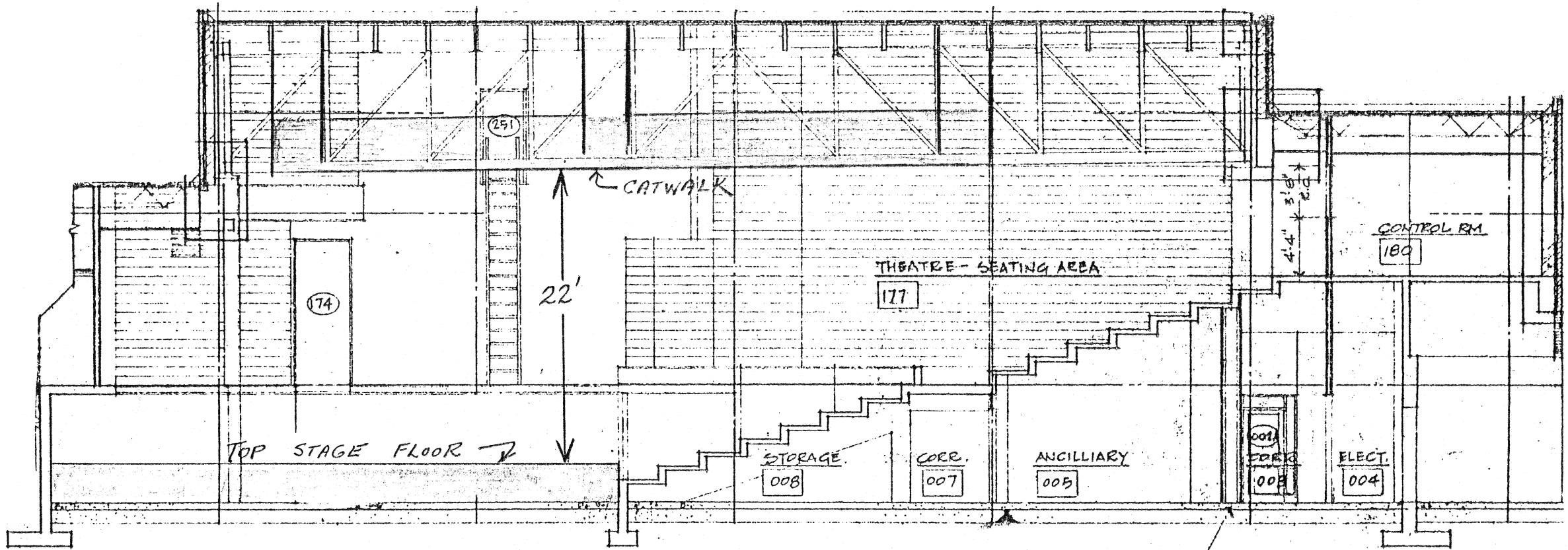
ELEVATION VIEW
